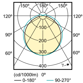
PLC /830, /840
