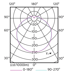
LEDtube 100mm 5W G24D-1
